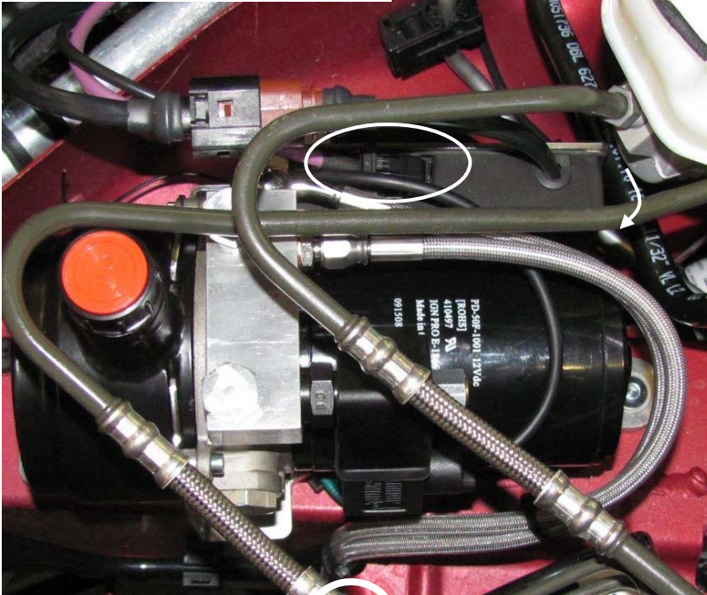
Montageposition 3 / Assembly position 3
