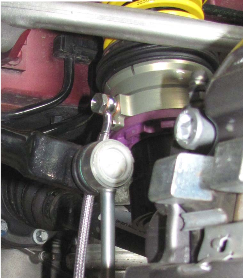
Montageposition 10 / Assembly position 10
