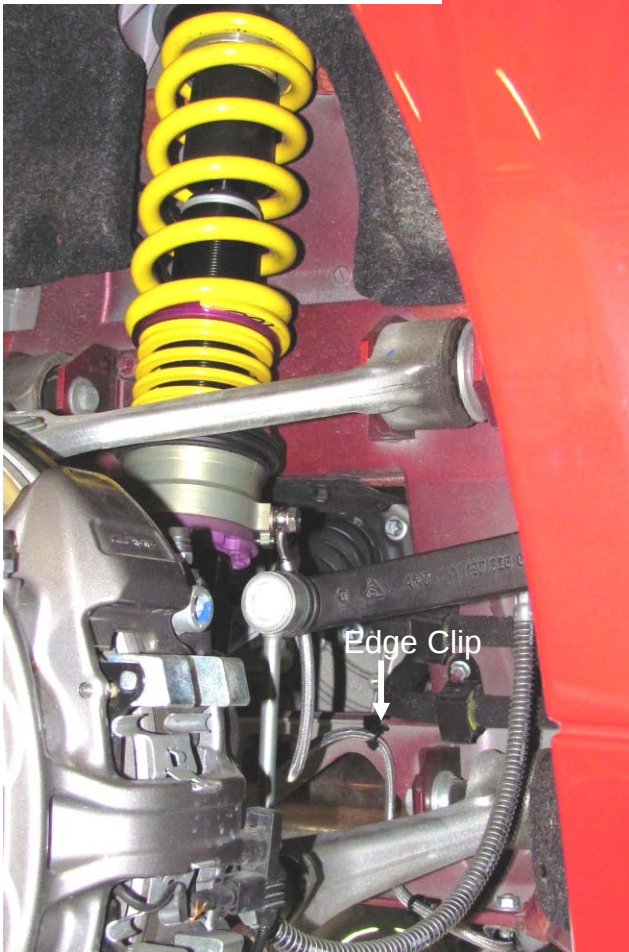
Montageposition 4 / Assembly position 4
