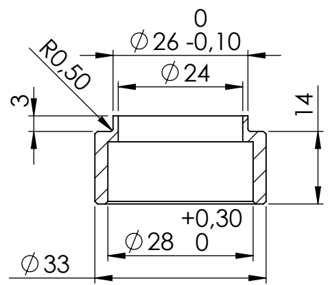
Bushing cod.206583
