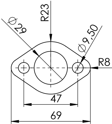
Flange 57F sp.6 mm cod.083457014
